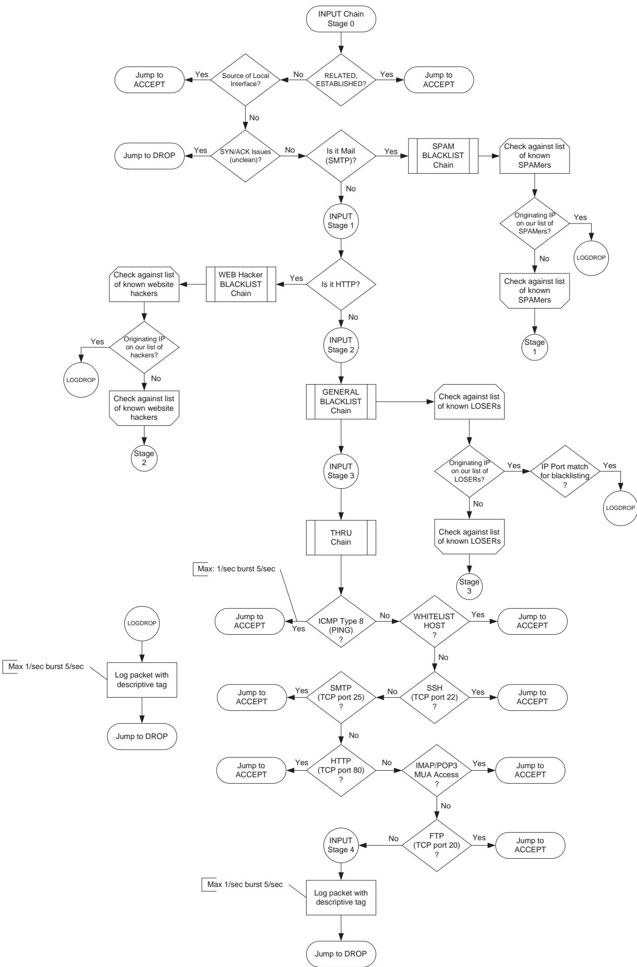
Example IPTABLES Configuration Flow Chart (c) Copyright Pettingers.org
